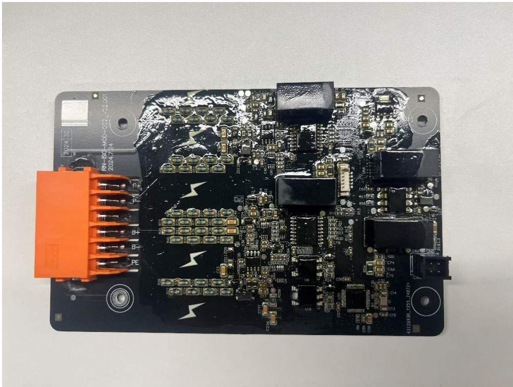
Figure 15 Front view of isolation board
