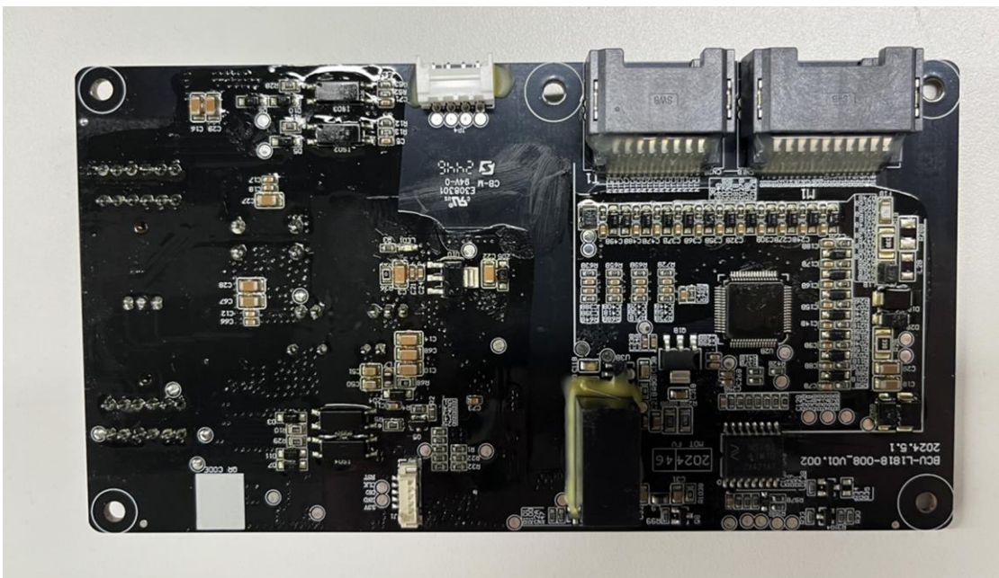
Figure 18 Back view of isolation board
