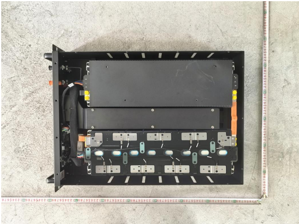
Figure 7 Inside view of battery module
