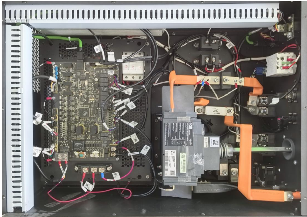
Figure 11 Inside view of HV box
