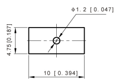
Terminal T4
