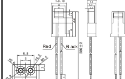
Connector H-Connector
