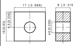
Terminal T10 Torque: 3.9 ~ 5.4 N*m
