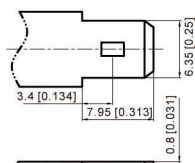
Terminal T2 FASTON TYPE
