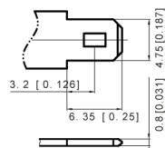
Terminal T1 FASTON TYPE
