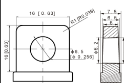
Terminal T5 Torque: 3.9 ~ 5.4 N*m
