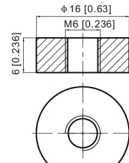
Terminal T6 Torque: 3.9 ~ 5.4 N*m
