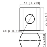
Terminal T9 Torque: 11 ~ 14.7 N*m
