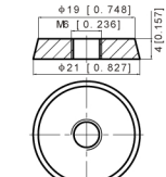
Terminal T13 Torque: 3.9 ~ 5.4 N*m
